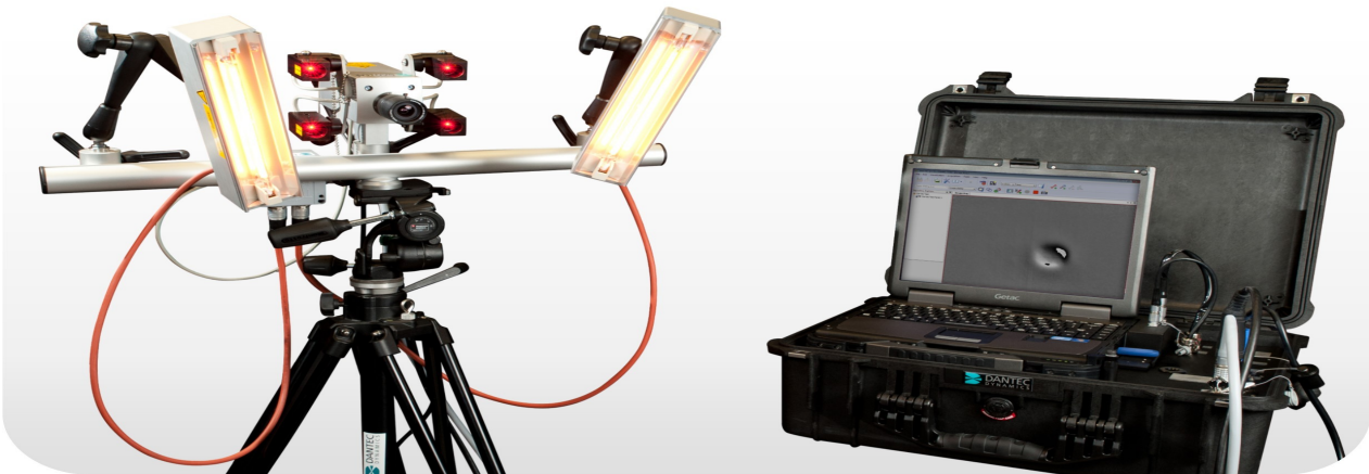
Figure 1 - Q-800 Portable Shearography System (with Automatic Heat Excitation)
